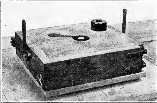
FIG. 532. VERTICAL GREEN-SAND CORE.
